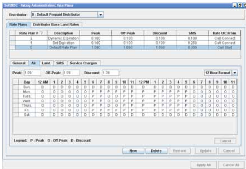
Rate Configuration Screen
